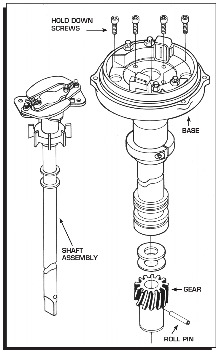
Figure 1 Disassembly.
