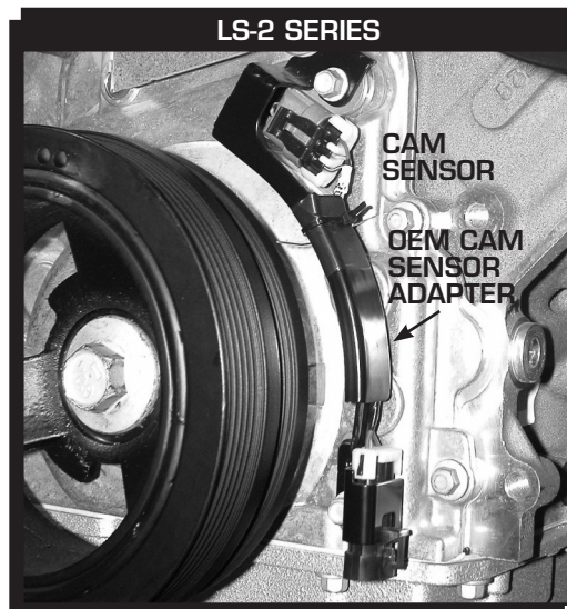
Figure 1 Camshaft Sensor Location.
