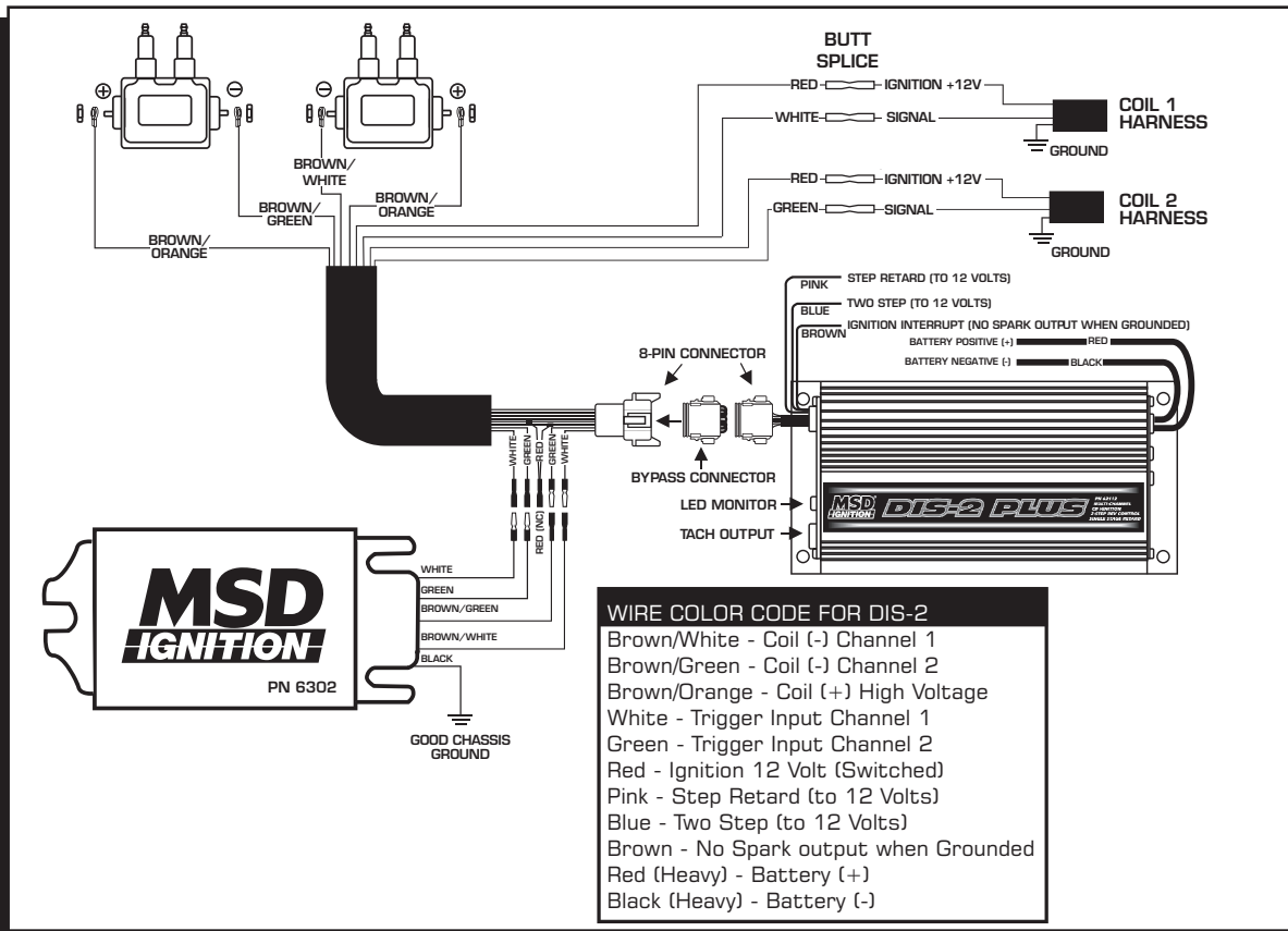
Figure 1 Wiring
