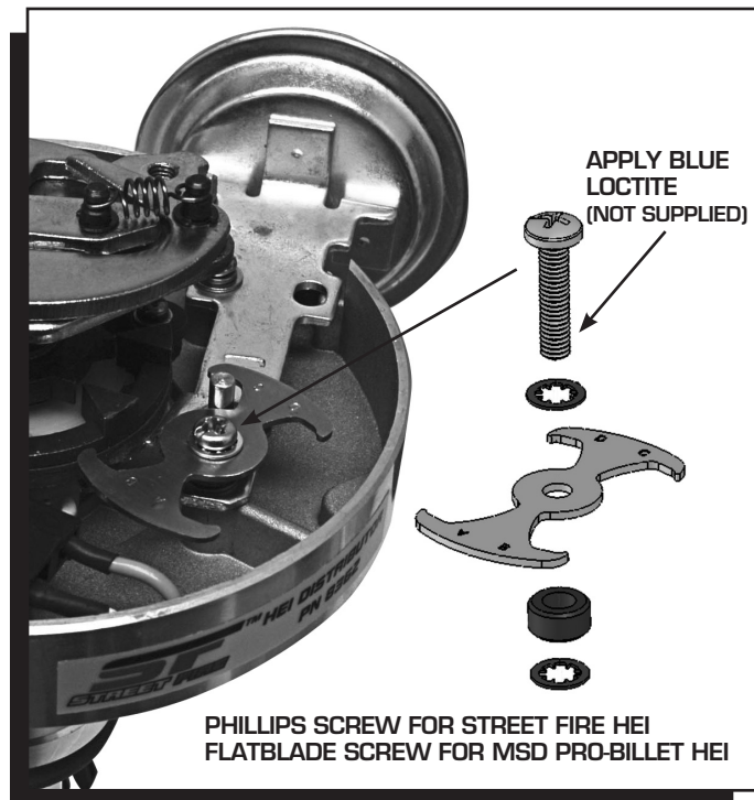
Figure 2 Installation.
